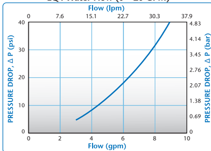
LQ4 Water Flow (0 – 20 GPM)
